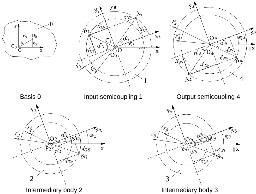
Fig. 2. The geometrical and kinematical multibody model
